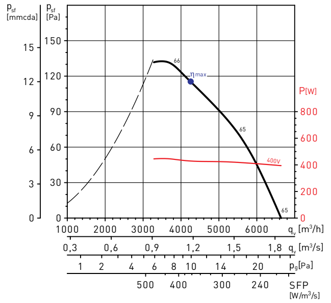
HCFT/4-450/H
