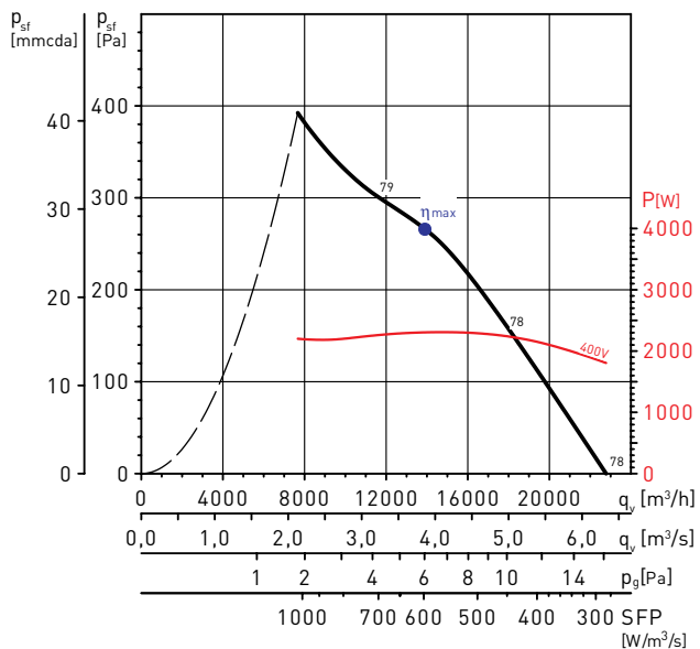
HCFT/4-800/L
