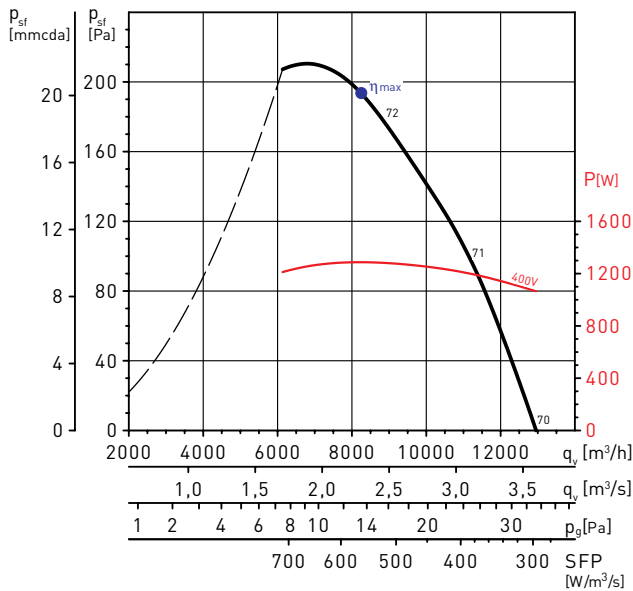
HCBT/4-560/H
