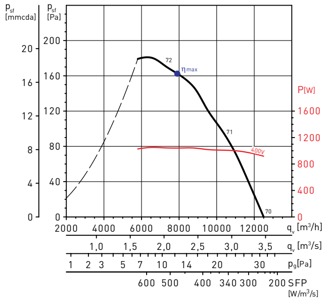
HCFT/4-560/H
