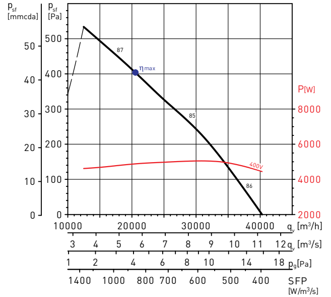
HCBT/4-1000/L
